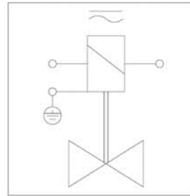
Anschlußplan / connection diagram
